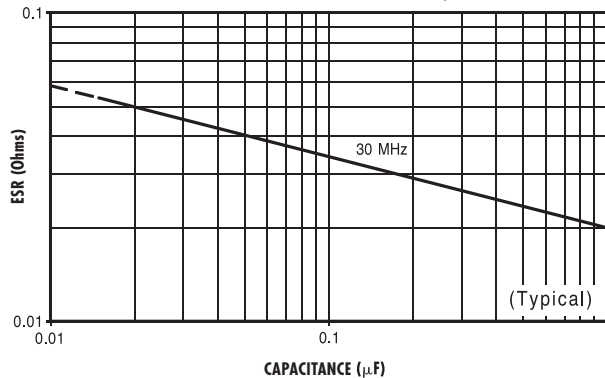
ESR VS CAPACITANCE ATC SERIES 900, CASE C
