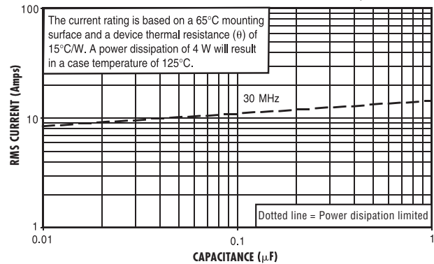
CURRENT RATING VS CAPACITANCE ATC SERIES 900, CASE C
